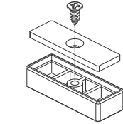
M3×6.8mm screw;/ Vis M3×6,8mm 30.6×10mm Magnet Catch/ 30,6×10mm Loquet magnétique 30.6×10mm Magnet Catch Base/ 30,6×10mm Base de loquet magnétique
